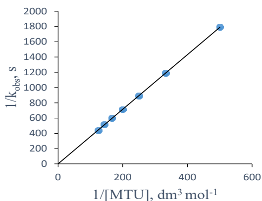
Fig. 3: Michealis-Menten plot of 1/k_{\text{obs}} versus 1/[\text{MTU}] for the oxidation of MTU by \text{Fe}_2\text{O}^{4+} at [\text{Fe}_2\text{O}^{4+}] = 2.0 \times 10^{-4} \text{ mol dm}^{-3} , [\text{MTU}] = (2.0 - 8.0) \times 10^{-3} \text{ mol dm}^{-3} , [\text{H}^+] = 1.0 \times 10^{-3} \text{ mol dm}^{-3} , I = 0.3 \text{ mol dm}^{-3} (NaCl), T = 27.0 \pm 1.0^\circ\text{C} and \lambda_{\text{max}} = 520
