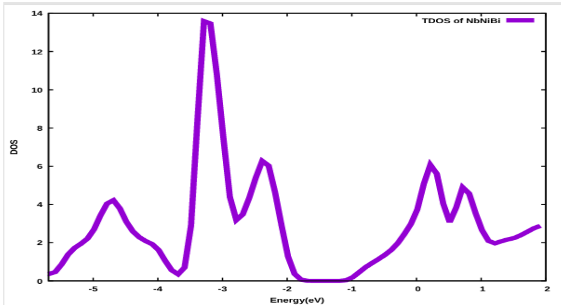
Fig. 3: Density of State of NbNiBi
