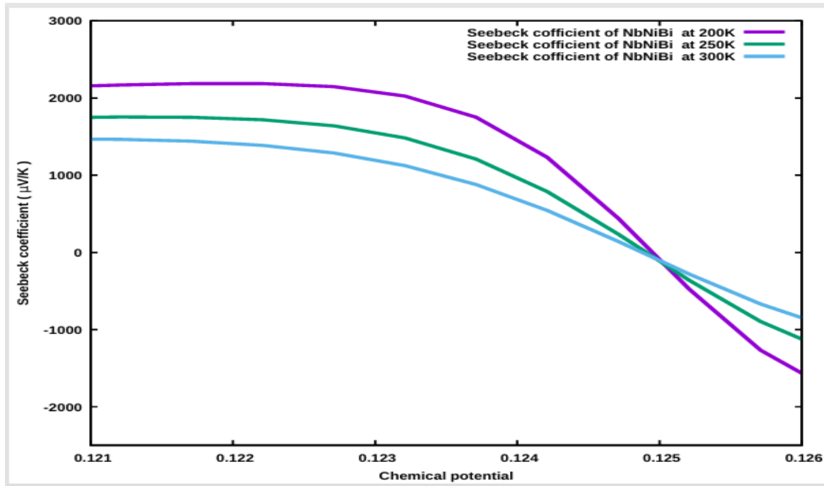
Fig. 5: Seebeck Coefficient of NbNiBi
