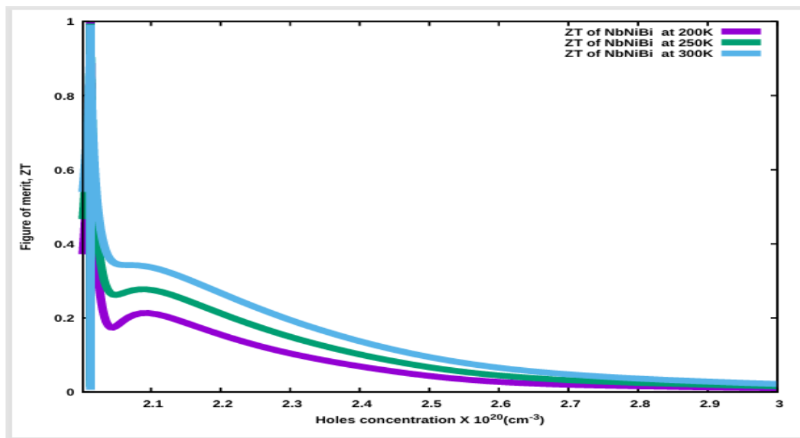
Fig. 6: Fig. of merit of NbNiBi
