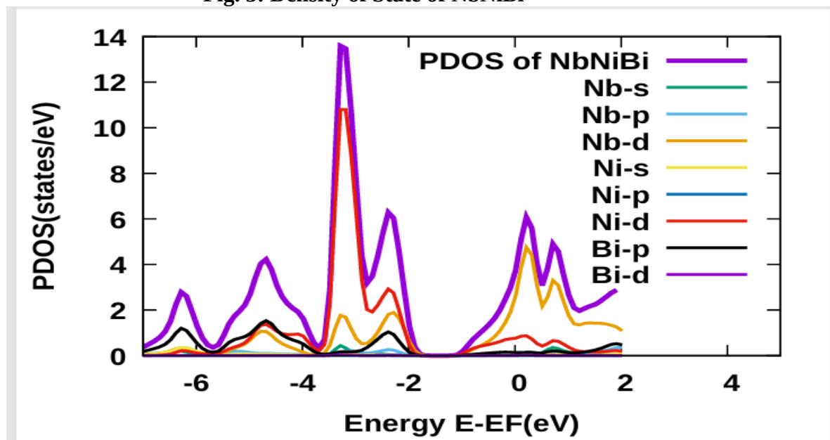
Fig. 4: Partial Density of State of NbNiBi
