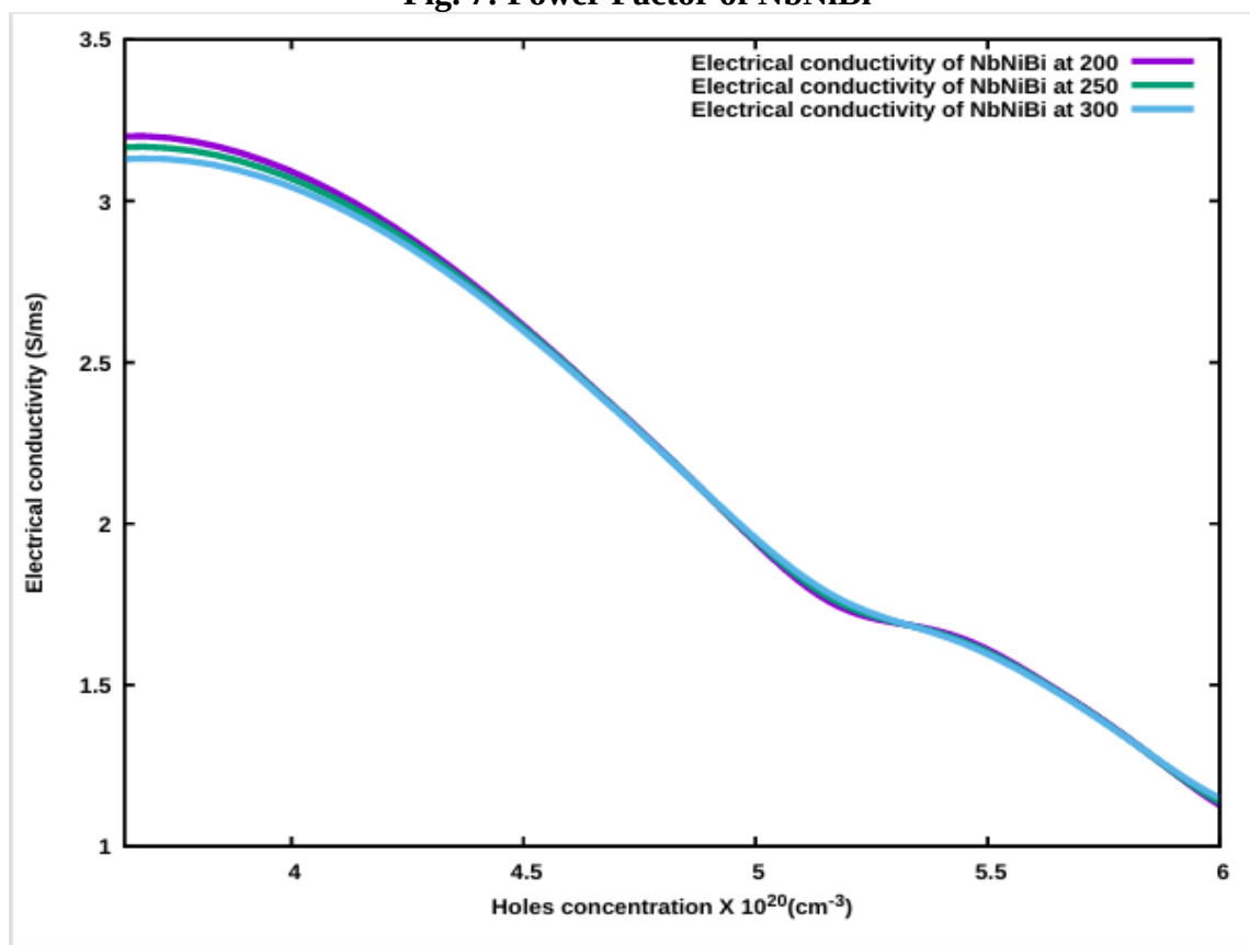
Fig. 8: Electrical conductivity of NbNiBi
