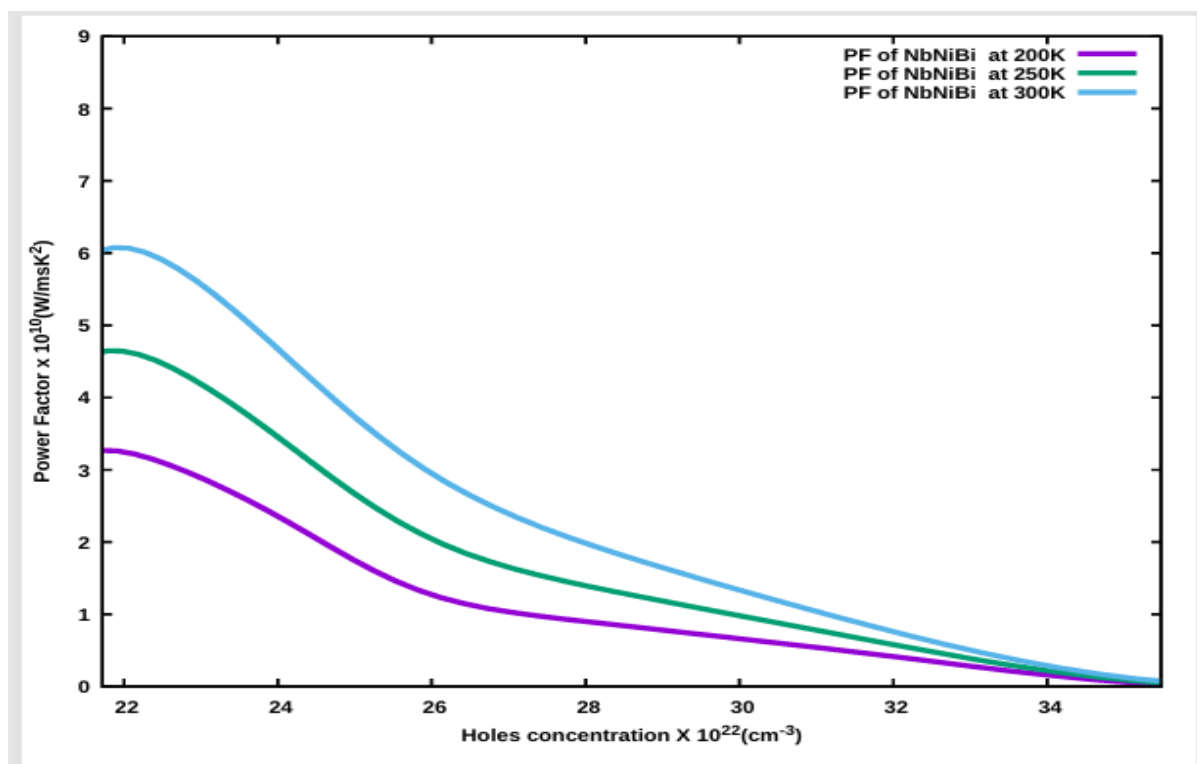
Fig. 7: Power Factor of NbNiBi
