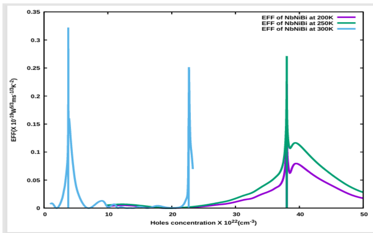
Fig. 9: Electronic Fitness Function of NbNiBi
