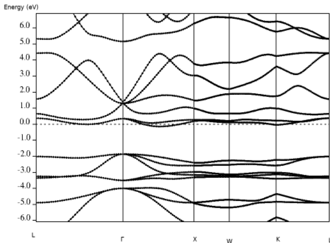
Fig. 2: Band energy of NbNiBi
